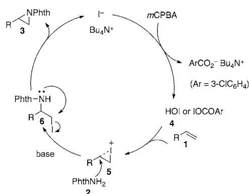
Scheme 1. Proposed mechanism of TBAI-catalyzed aziridination.
