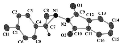
Figure 1. X-ray crystal structure of N -(aminophthalimide)-2-(4-chlorophenyl)aziridine ( 3e ). Thermal ellipsoids are shown at 50% probability and some hydrogen atoms have been omitted for clarity.
